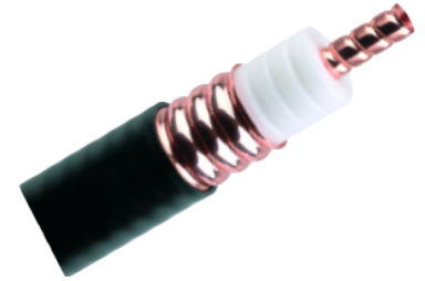
7/8" CELLFLEX® Ultra-Flexible Low-Loss Foam Dielectric Coaxial Cable
